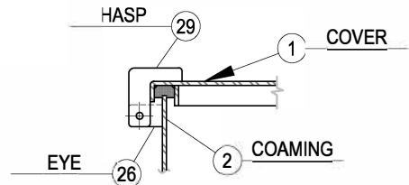
DETAIL OF HASP & EYE
